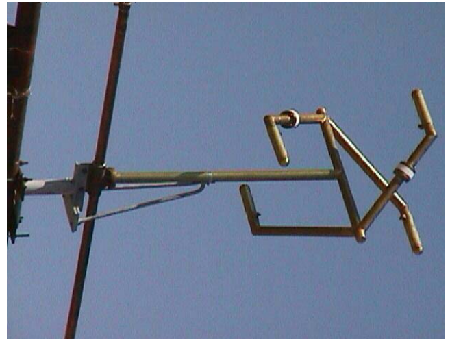
1-5/8" OD Element Thick Wall Construction
