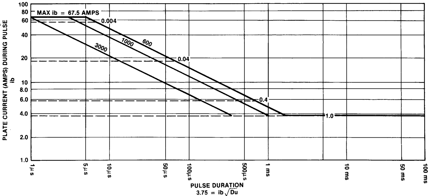
PULSE DERATING CHART, PULSE MODULATOR OR REGULATOR SERVICE
