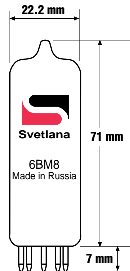
Outline Drawing 6BM8 Triode and Pentode
