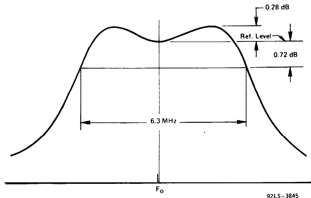
Figure 2 - Bandwidth Characteristics
