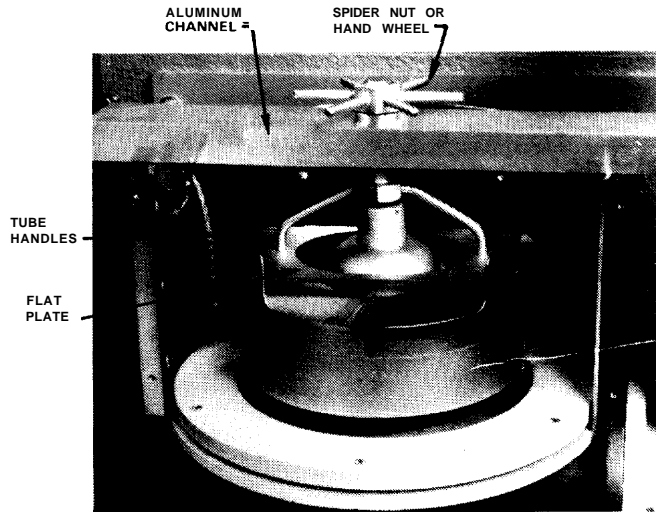
Figure 9 - BURLE Tube Type 8807 Being Removed
