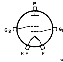
Figure 8 - Terminal Diagram
